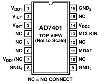
Figure 5. Pin Configuration
